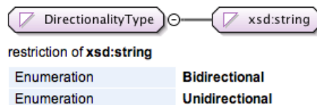
Figure 147 – DirectionalityType .
