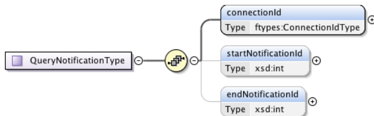
Figure 105 – QueryNotificationType.
