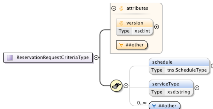
Figure 117 – ReservationRequestCriteriaType .
