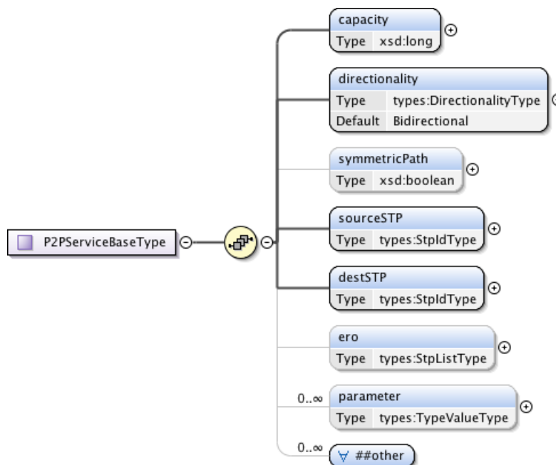
Figure 138 – P2PServiceBaseType.
