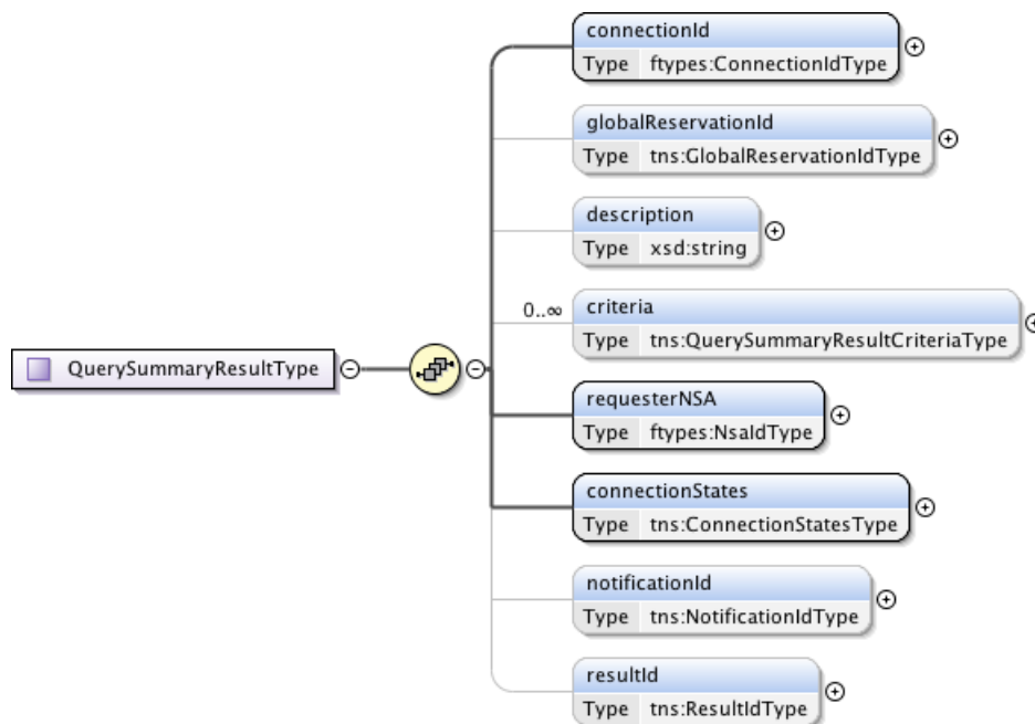
Figure 114 – QuerySummaryResultType.
