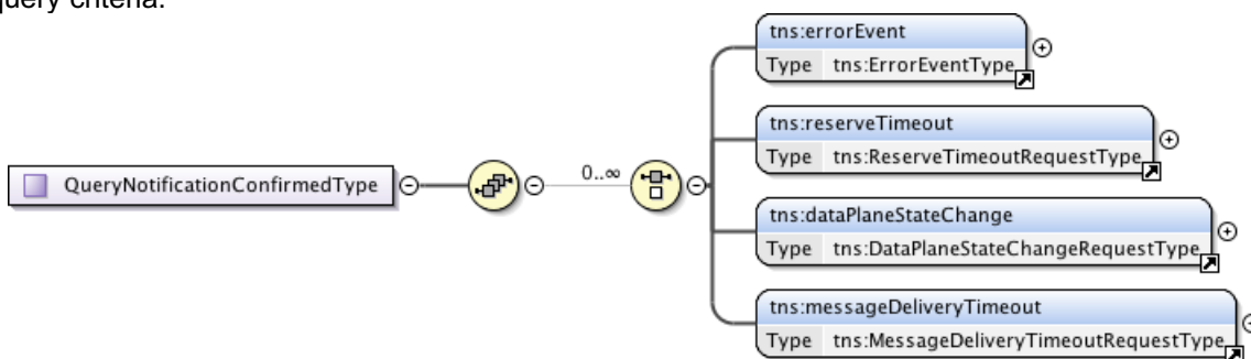
Figure 104 – QueryNotificationConfirmedType.
