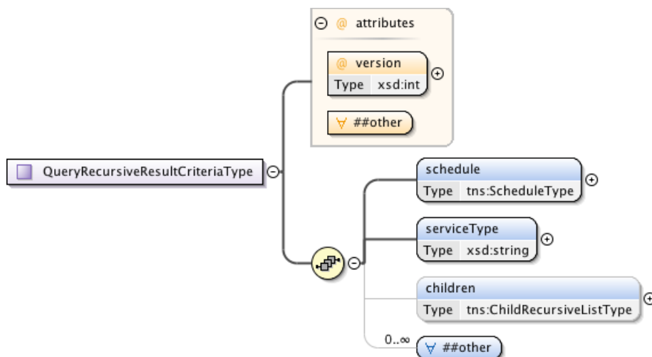
Figure 107 – QueryRecursiveResultCriteriaType.
