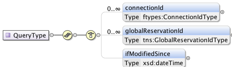
Figure 115 – QueryType.
