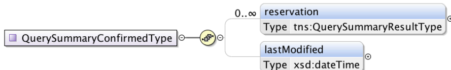
Figure 112 – QuerySummaryConfirmedType.
