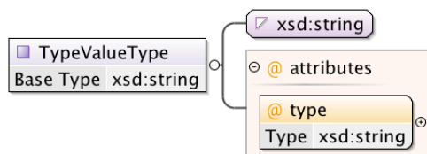
Figure 141 – TypeValueType.
