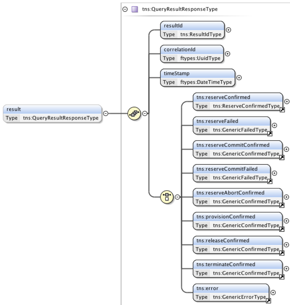
Figure 84 – QueryResultResponseType structure.
