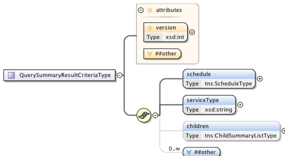
Figure 113 – QuerySummaryResultCriteriaType.
