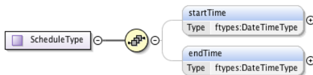
Figure 122 – ScheduleType.
