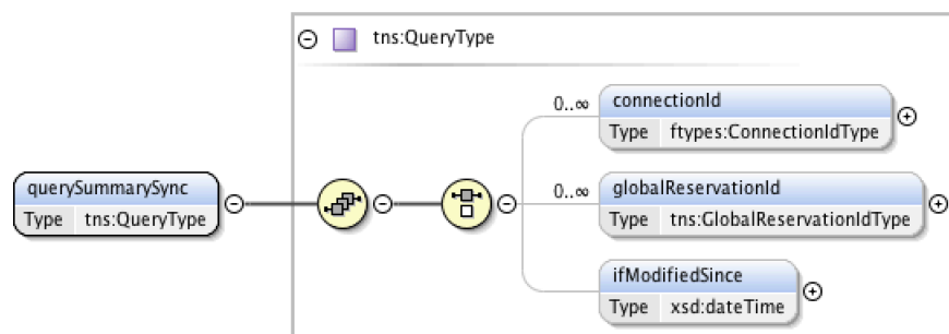
Figure 69 – querySummarySync request message structure.
