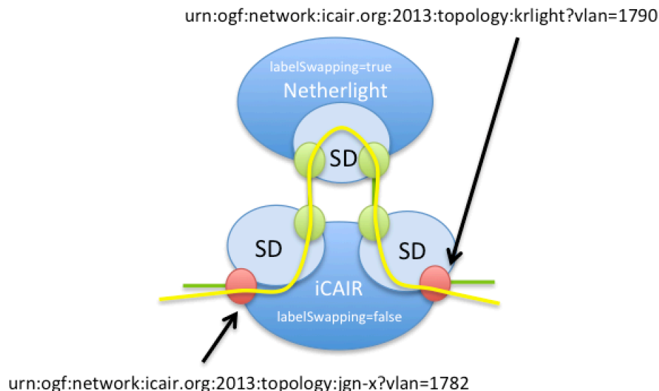
Figure 158 – Unnecessary Connection loops.
