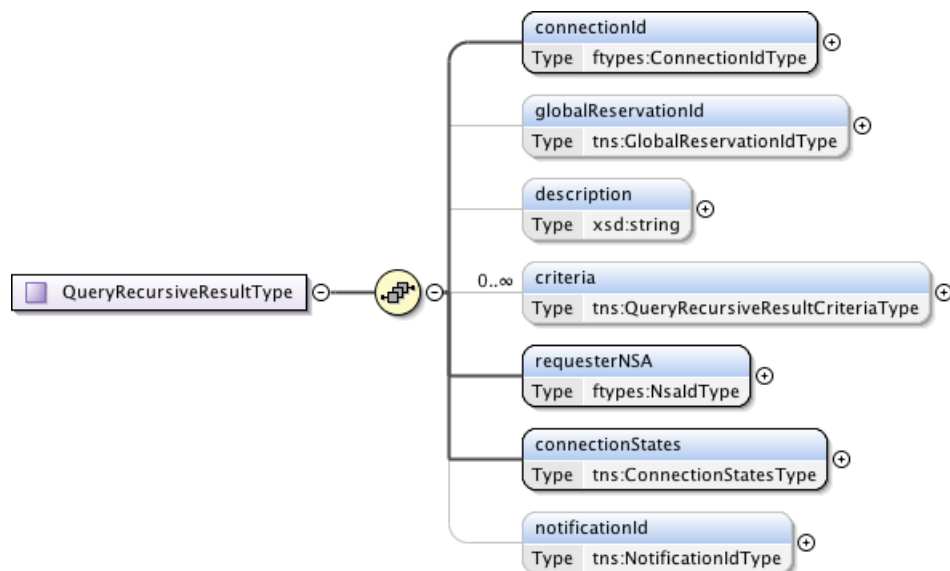
Figure 108 – QueryRecursiveResultType.
