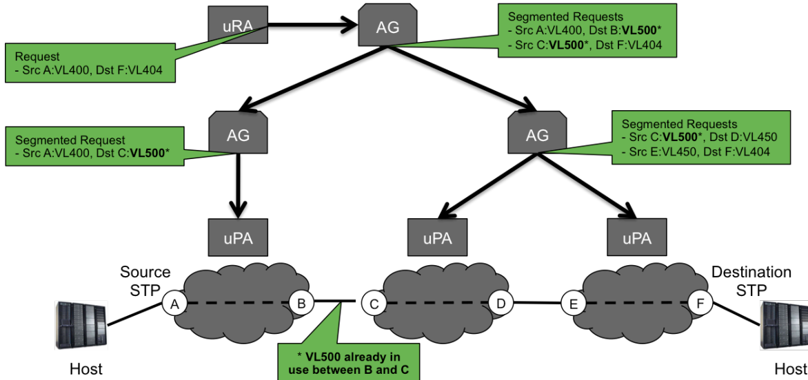
Figure 151: Example VLAN selection collision in Tree Connection workflow.
