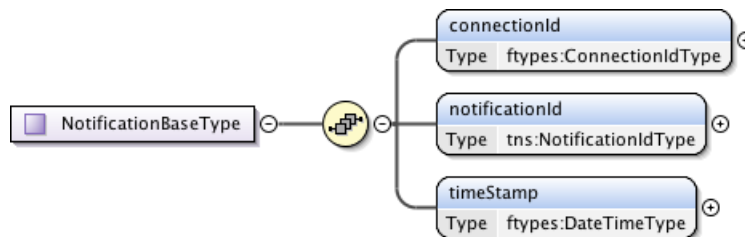
Figure 103 – NotificationBaseType.
