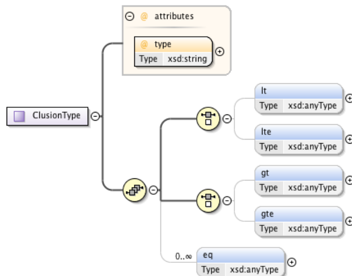
Figure 142 – ClusionType .
