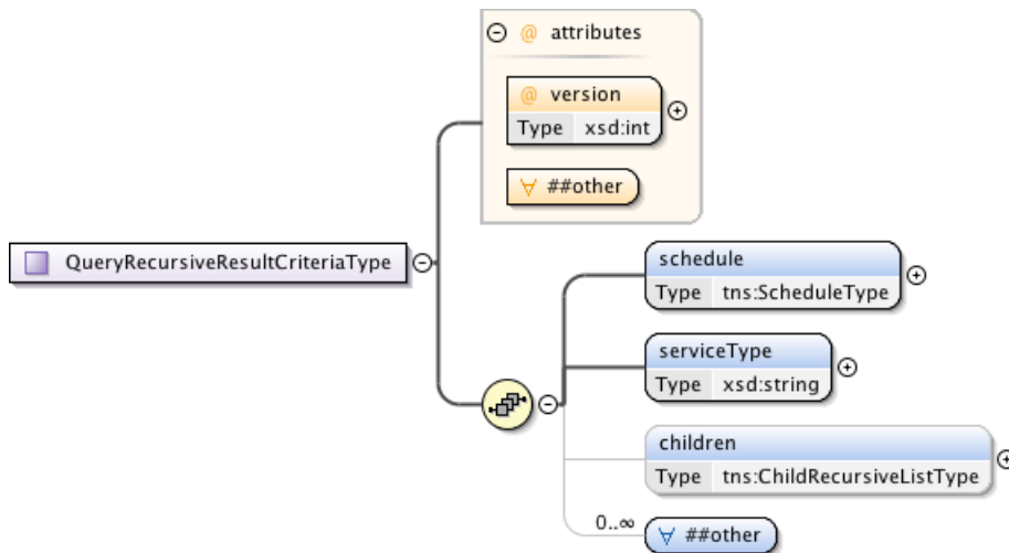
Figure 107 – QueryRecursiveResultCriteriaType.
