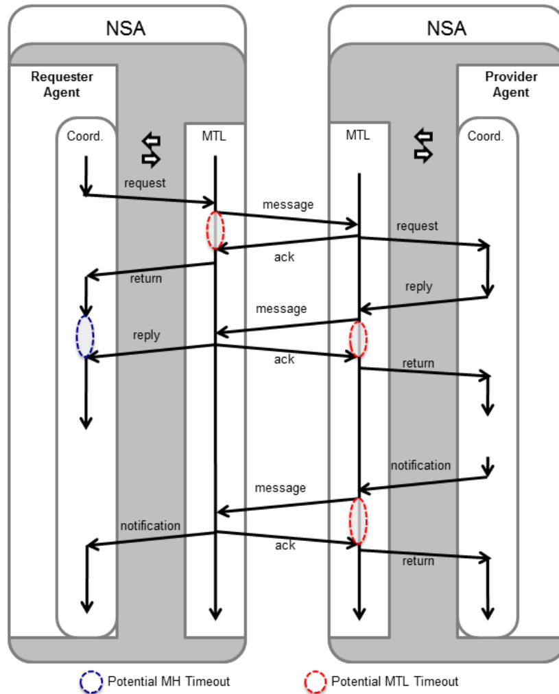
Figure 130: Potential MH/MTL timeout sequences
