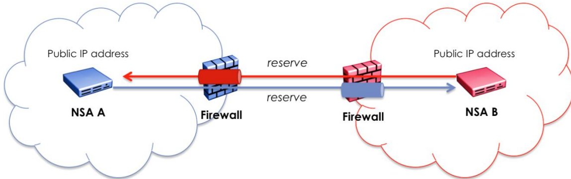
Figure 133 – Peer NSA behind a firewall with public IP addresses.
