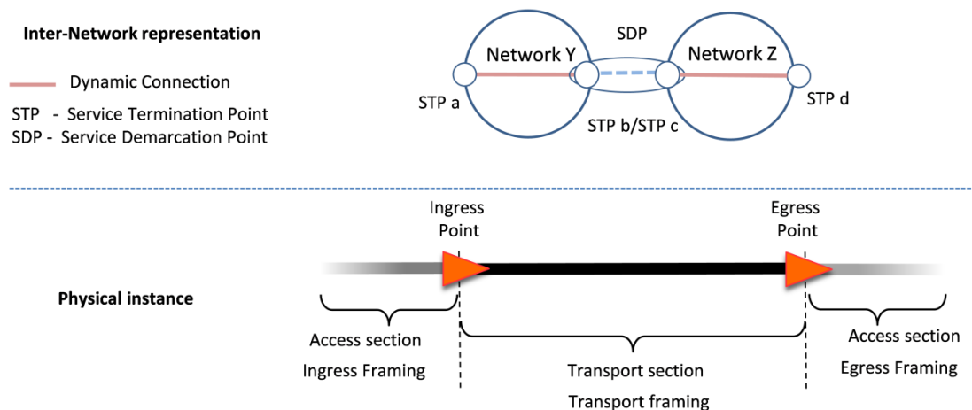
Figure 1: Inter-Network representation of a Connection
