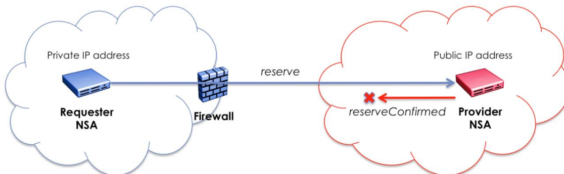
Figure 131 – RA behind a firewall with private IP address.
