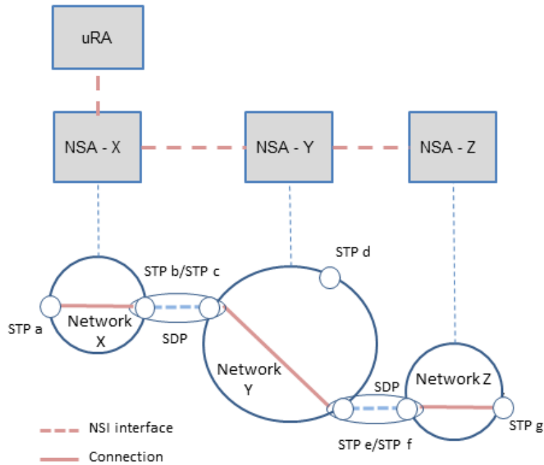
Figure 143: Example of Connection managed by an NSA chain
