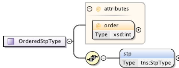
Figure 139 – OrderedStpType.
