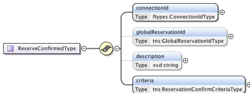
Figure 118 – ReserveConfirmedType.
