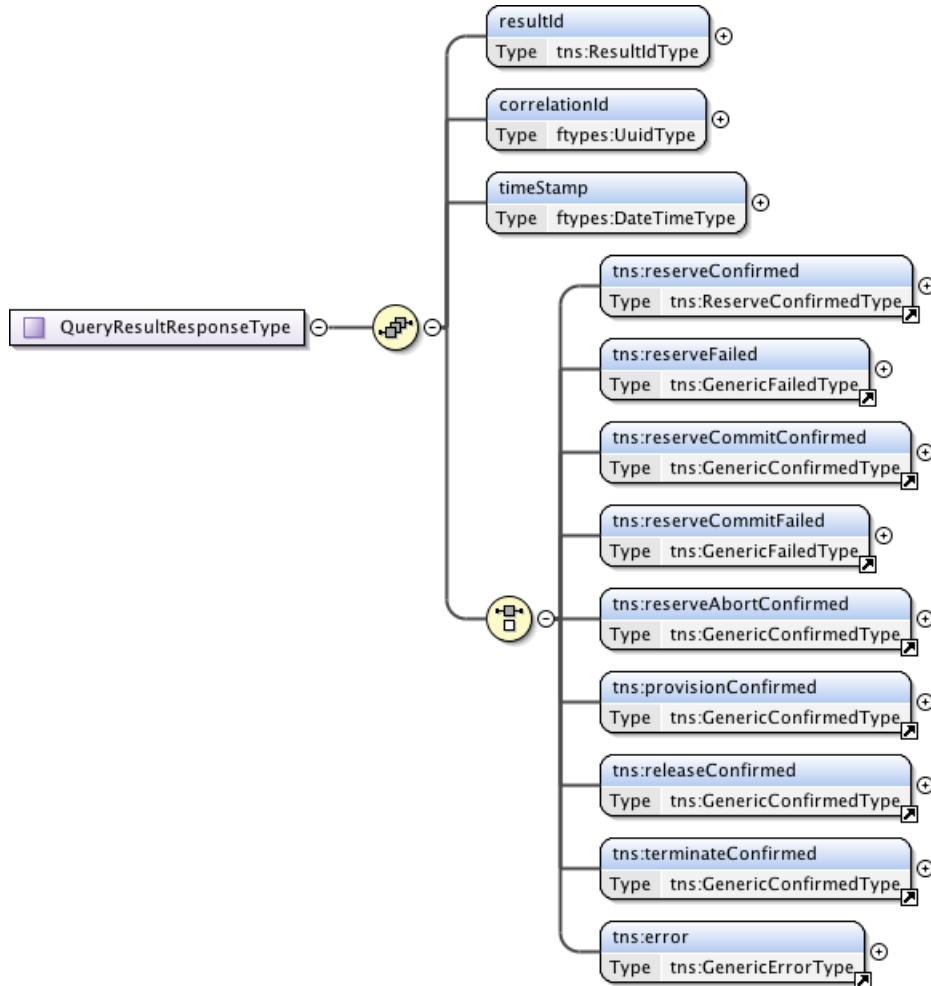
Figure 110 – QueryResultResponseType structure.
