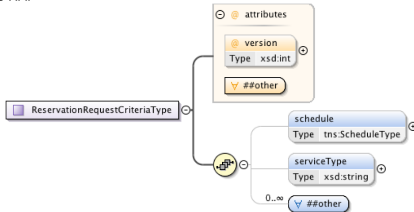
Figure 117 – ReservationRequestCriteriaType.
