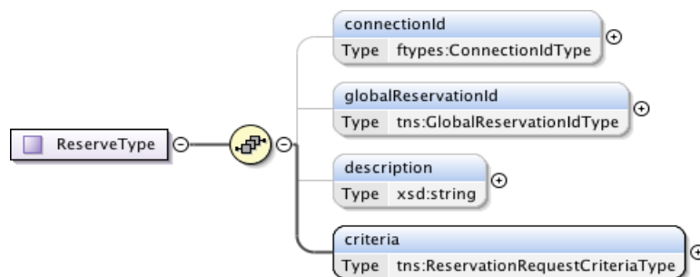
Figure 121 – ReserveType.
