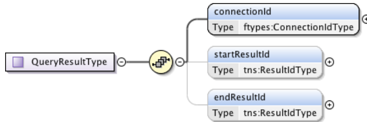
Figure 111 – QueryResultType.
