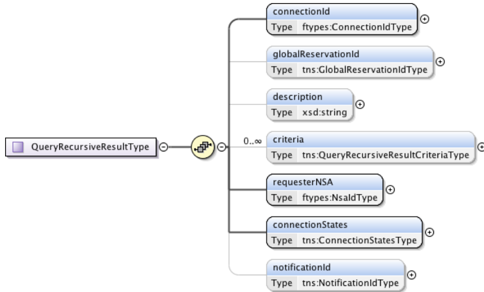
Figure 108 – QueryRecursiveResultType.
