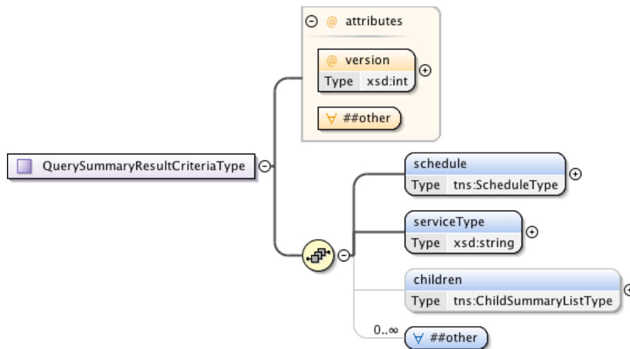
Figure 113 – QuerySummaryResultCriteriaType .
