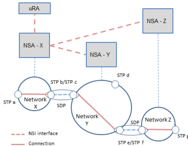
Figure 144: Example of a Connection managed by a NSA tree
