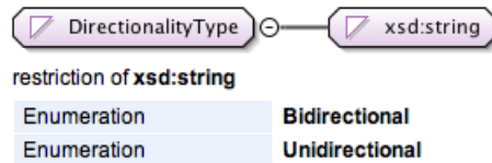
Figure 142 – DirectionalityType .
