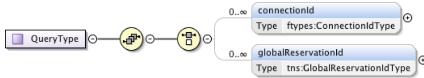
Figure 115 – QueryType.
