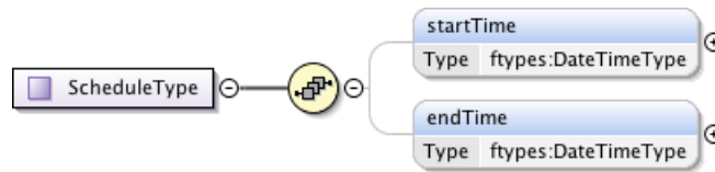
Figure 122 – ScheduleType .
