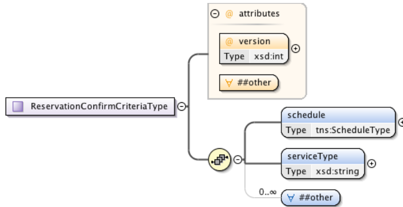
Figure 116 – ReservationConfirmCriteriaType.
