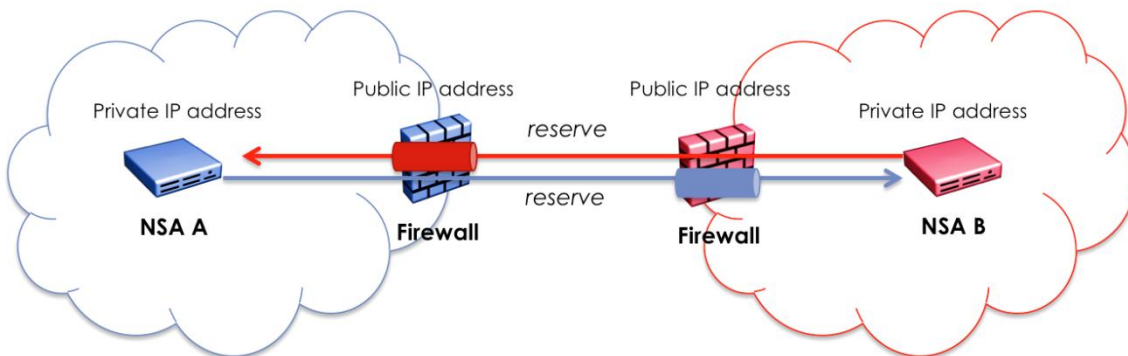
Figure 134 – Peer NSA behind a firewall with private IP addresses.
