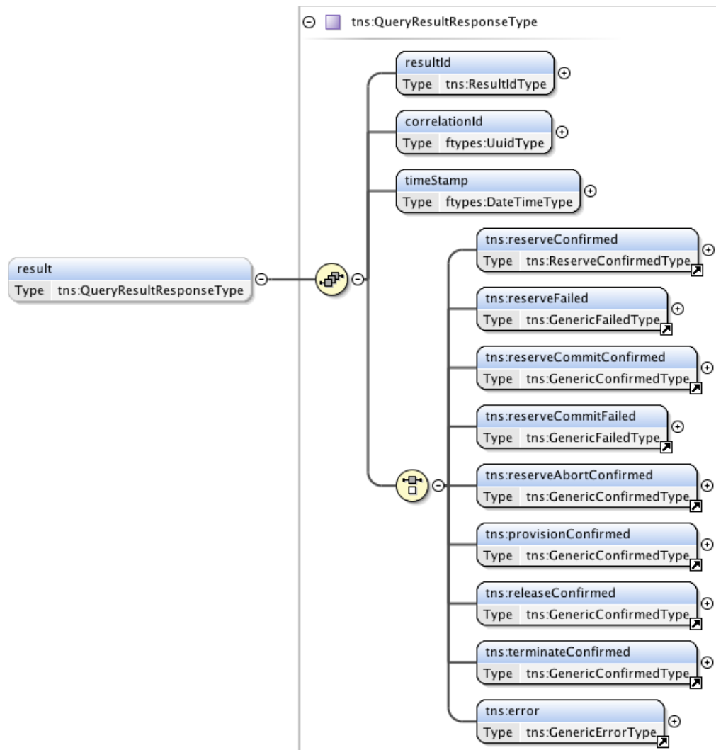
Figure 84 – QueryResultResponseType structure.
