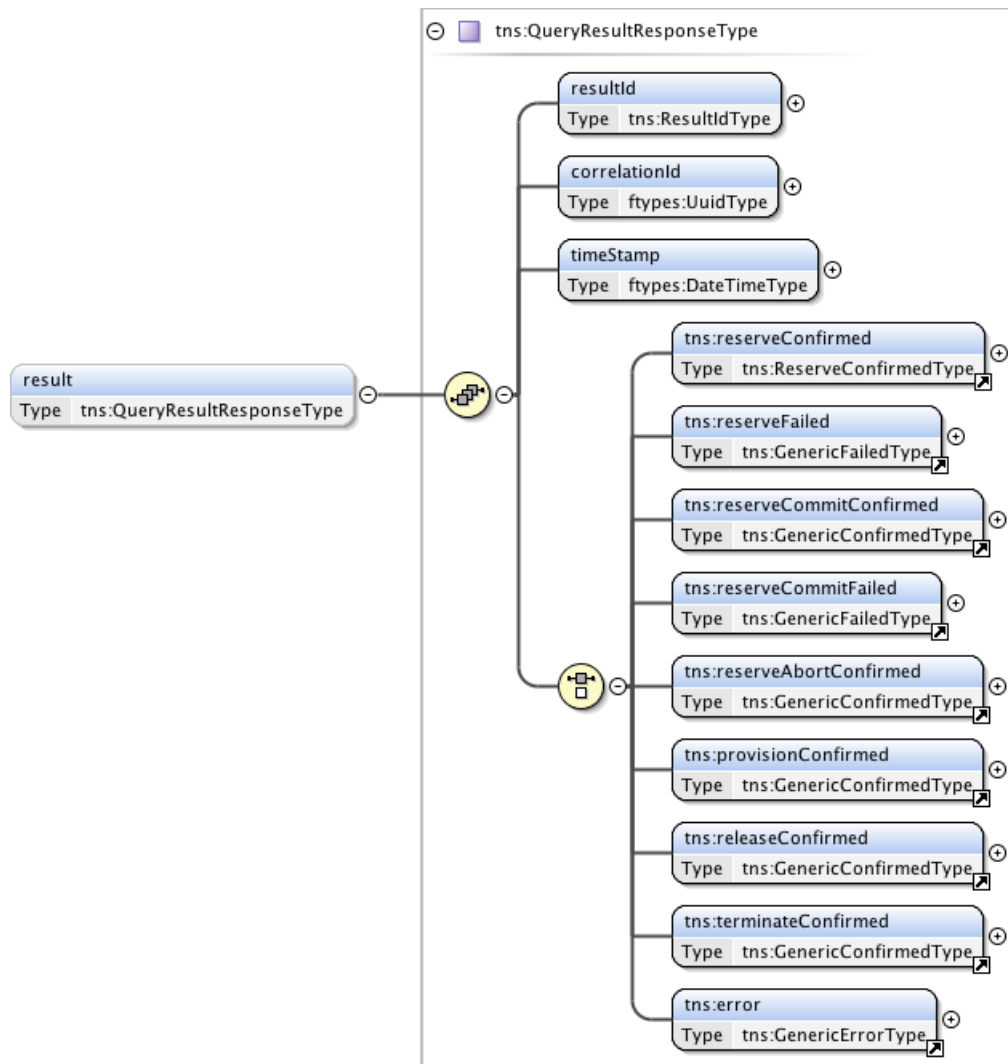
Figure 88 – QueryResultResponseType structure.
