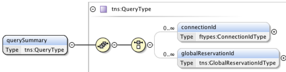
Figure 65 – querySummary request message structure.
