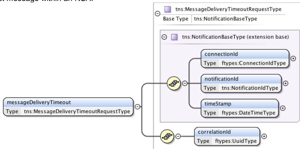
Figure 63 – messageDeliveryTimeout request message structure.
