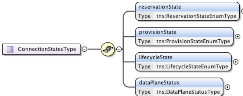
Figure 93 – ConnectionStatesType .
