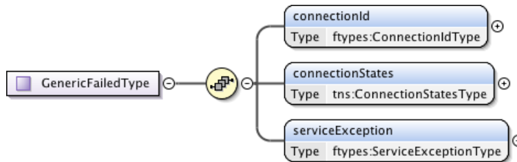
Figure 100 – GenericFailedType .
