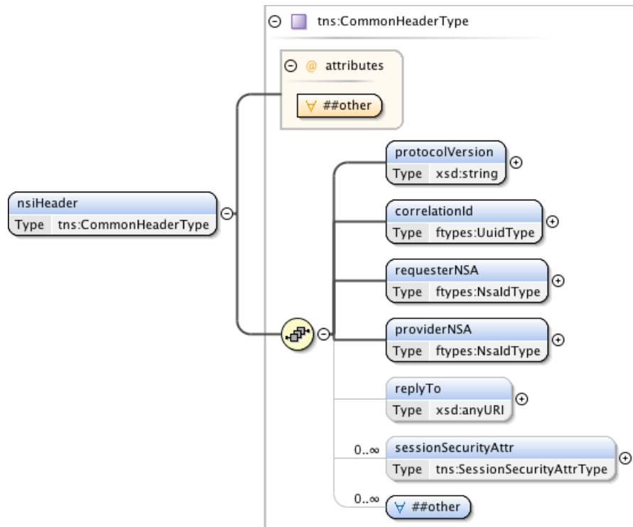
Figure 17 – nsiHeader structure.
