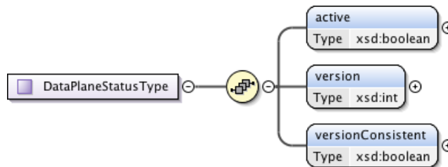
Figure 95 – DataPlaneStatusType.
