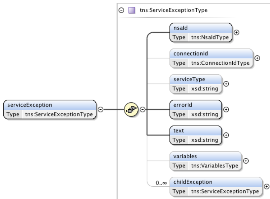
Figure 19 – ServiceExceptionType type.
