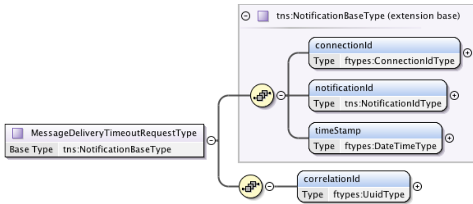
Figure 102 – MessageDeliveryTimeoutRequestType.
