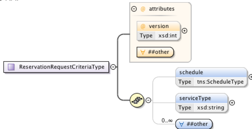
Figure 118 – ReservationRequestCriteriaType.
