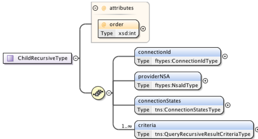
Figure 90 – ChildRecursiveType.
