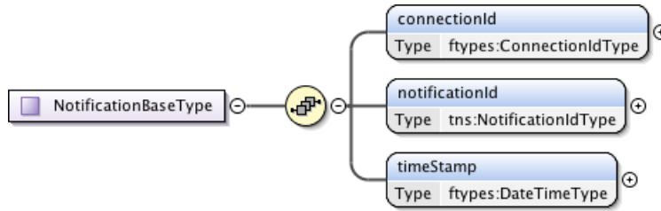
Figure 103 – NotificationBaseType.
