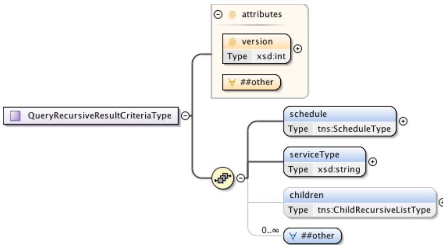
Figure 108 – QueryRecursiveResultCriteriaType .
